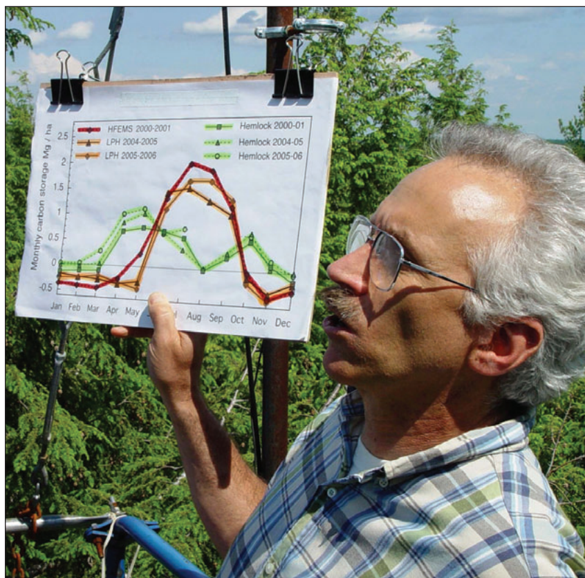
Figure 3. Telling a compelling ecological story requires quantitative data. Here, Harvard Forest researcher Julian Hadley describes monthly cycles of carbon storage in hemlock and hardwood stands. The data are collected at 10–20 Hz from three eddy-covariance towers, analyzed and summarized with time-series modeling, and incorporated into regional estimates (eg Matross et al. 2006) and forecasts (eg Desai et al. 2007), and used to determine regional and national carbon emissions targets and policies. Photo used with permission from the Harvard Forest Archives.
